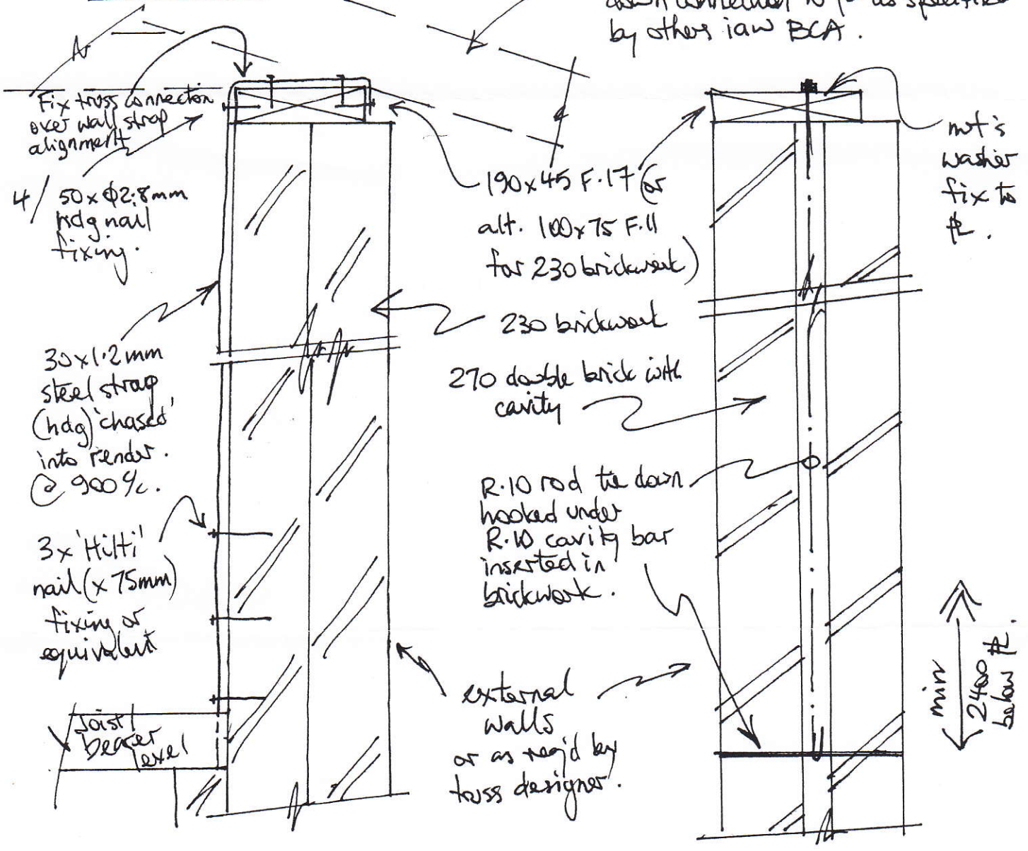
TYPICAL TOP \# TIE DOWN SECTIONS.
