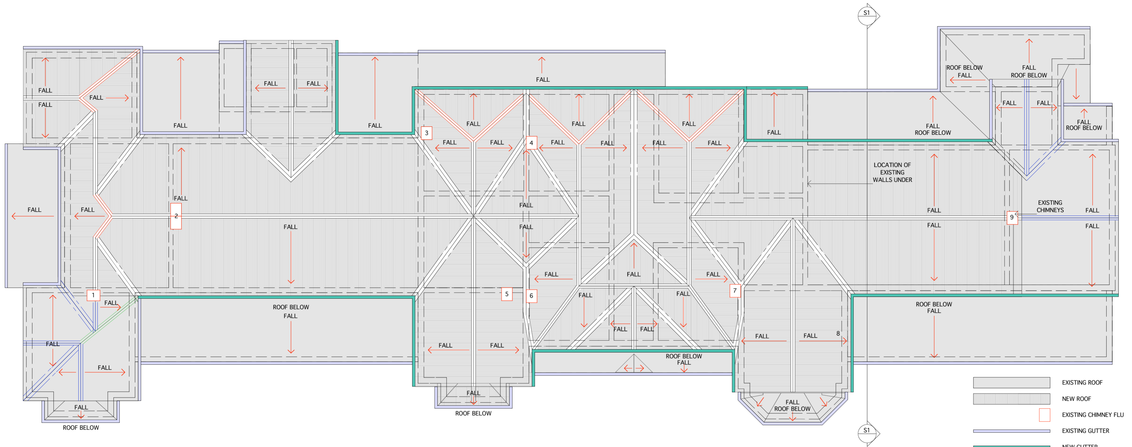
ROOF PLAN 1:100
